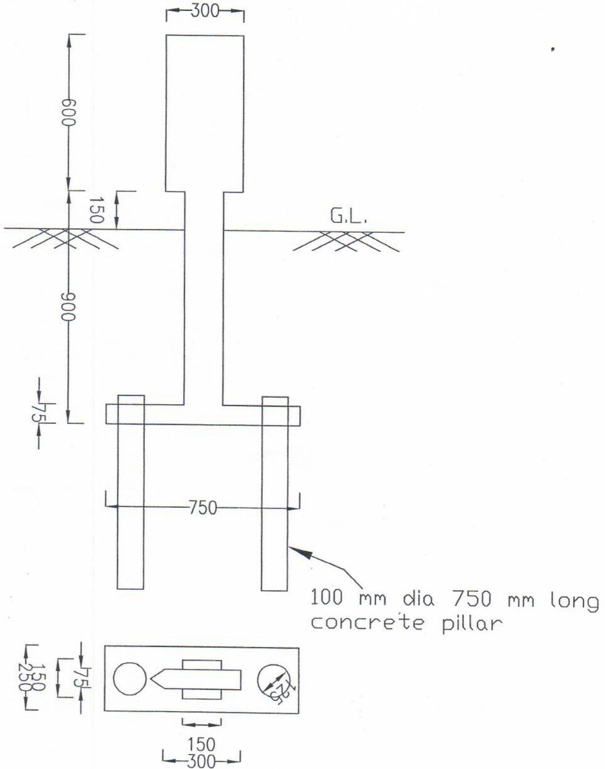
DRAWING OF BOUNDARY PILLAR
